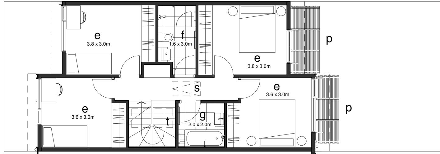
first floor
