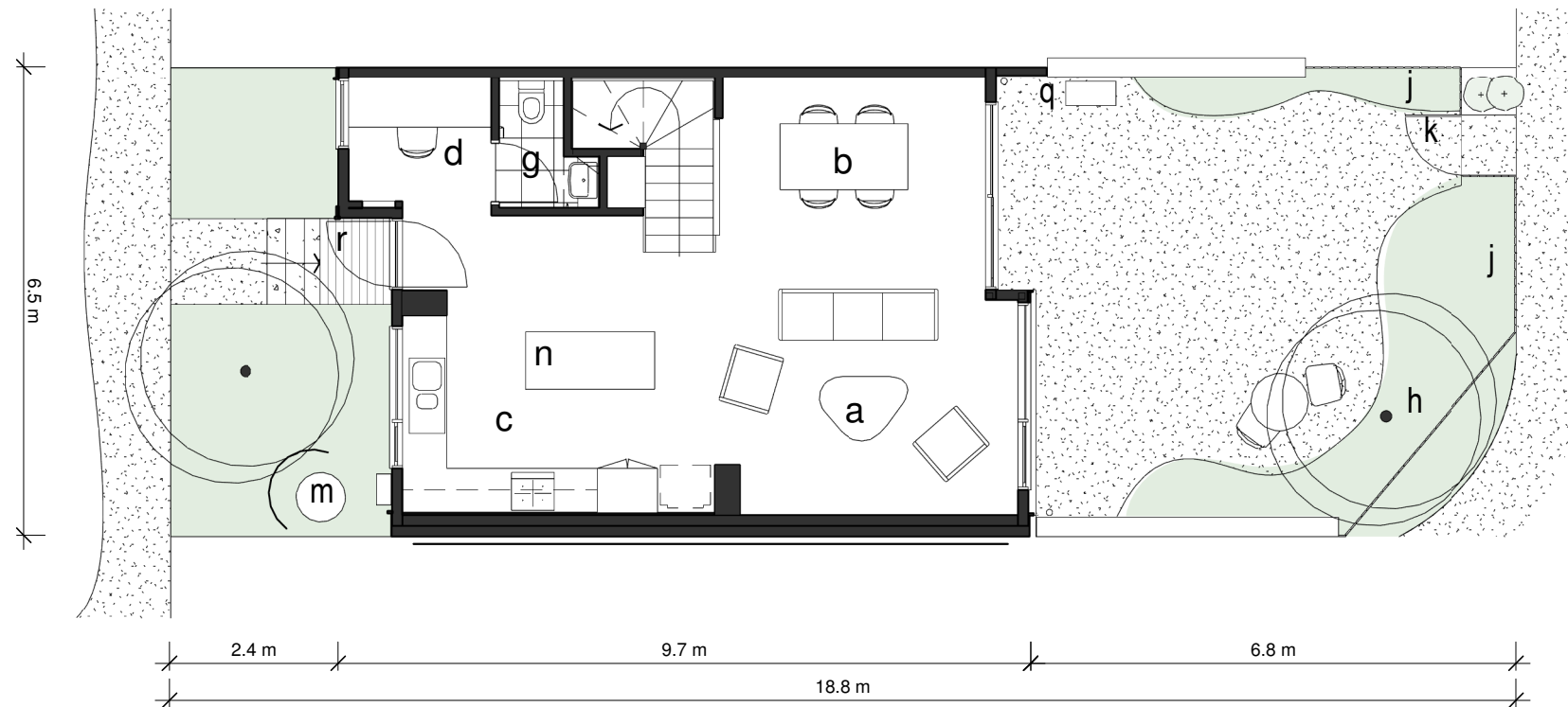
ground floor
